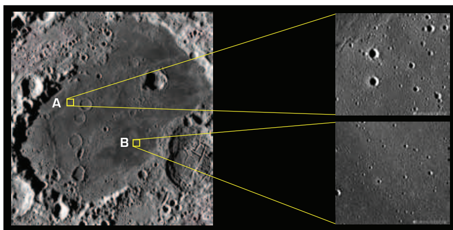
Chronology of Mare Moscoviense on the lunar farside. The Terrain Camera aboard KAGUYA provides high-resolution images to sufficiently detect small craters. As a result of crater counting by TC observation data, several areas of Mare Moscoviense show their younger ages. Area B is 1 billion years younger than area A. Area B had been active until 2.5 billion years ago.
