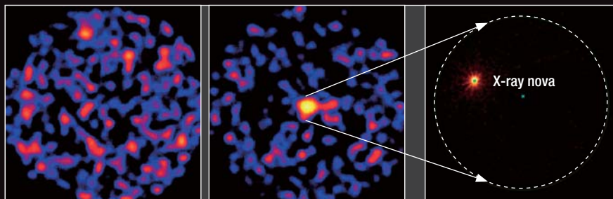
a: Prior to the appearance of the nova observed by MAXI (January 7, 2011)
