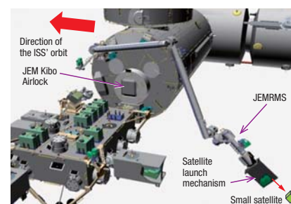
JEM Kibo's satellite-launch function
