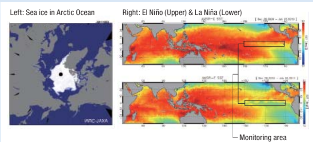
AMSR-E observation examples
