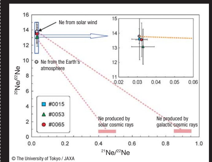
Neon emitted from the sun was present in the three Itokawa sample particles analyzed (#0015, #0053, and #0065)
