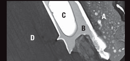
Many Itokawa Particles Show Evidence of Catastrophic Impacts
