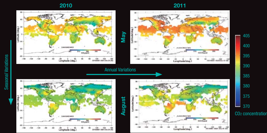
Global Distribution of CO 2 Concentration Based on Observations by GOSAT in May and August 2010 and 2011
