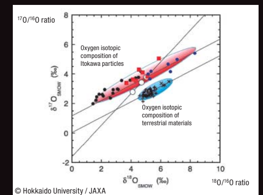
Comparison of the Oxygen Isotopic Composition of Itokawa Particles and Terrestrial Materials Reveals that the Itokawa particles have a different origin to terrestrial matter
