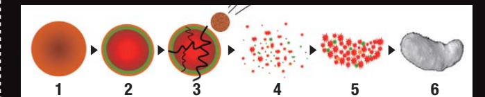
History of Itokawa's Formation
