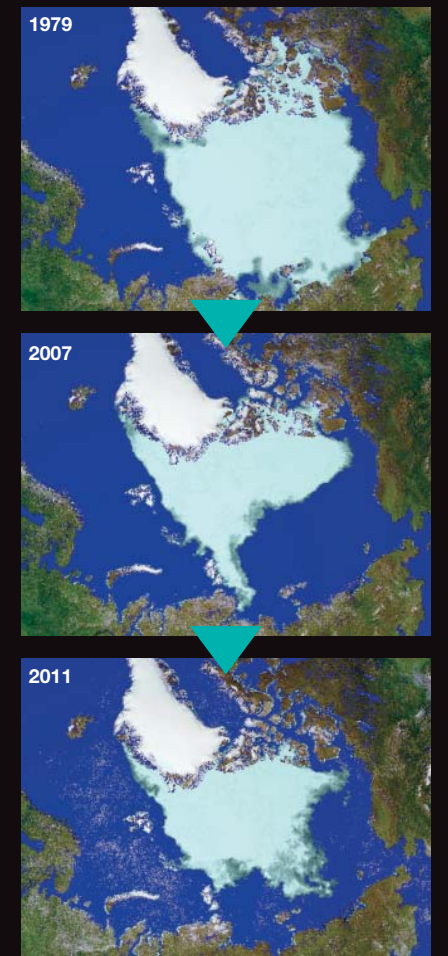
Distribution of Arctic Sea Ice Observed by AMSR-E
