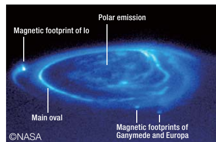
An image of Jupiter's northern ultraviolet aurorae captured by the Hubble Space Telescope
