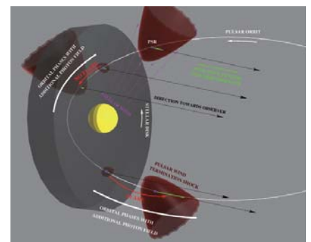
Sketch of interaction in binary pulsar system. Image credit: ApJL
