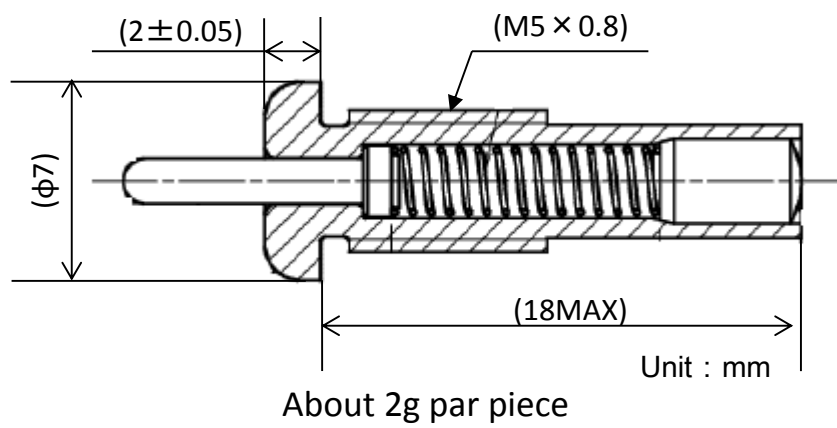
Figure C3-3 Spring Plunger
